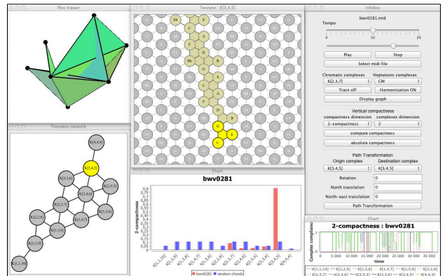
Figure 9. Graphical user interface of HexaChord.
